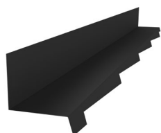
SCRIBED SIDE WALL FLASHING 320 (L)
